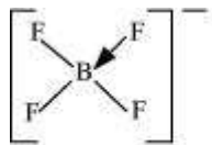
Tetrahedral structure
